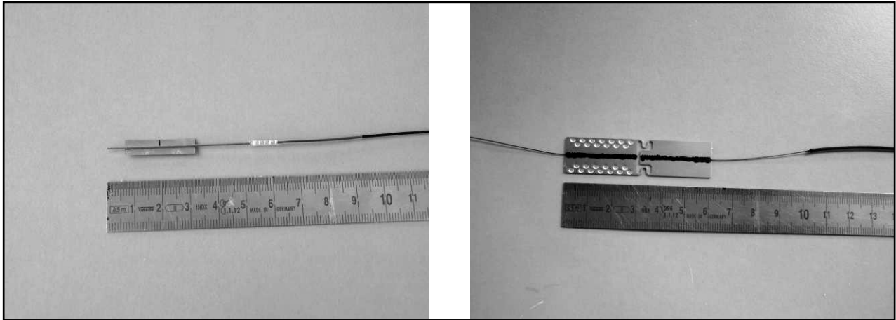
Figure 4. Fibre Optic strain sensors, FP left, FBG right.
