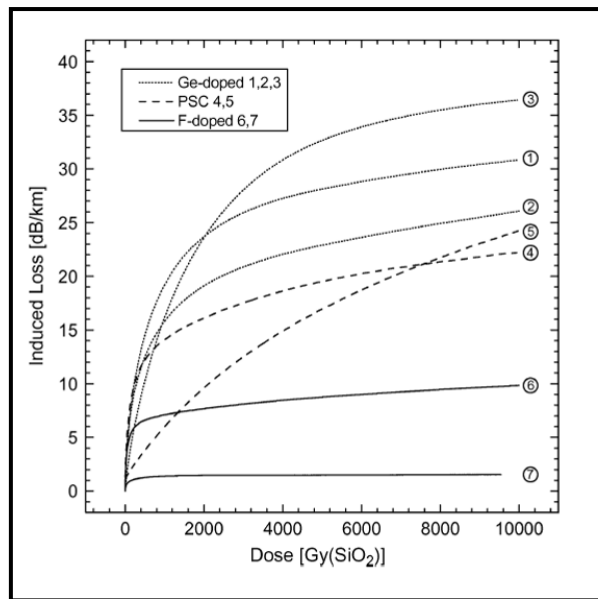
Figure 12. Induced losses in commercial radiation-hard fibres according to the radiation dose (Co-60). Fluorine-doped fibres (curves 6 and 7) show almost no change in optical transmission.
