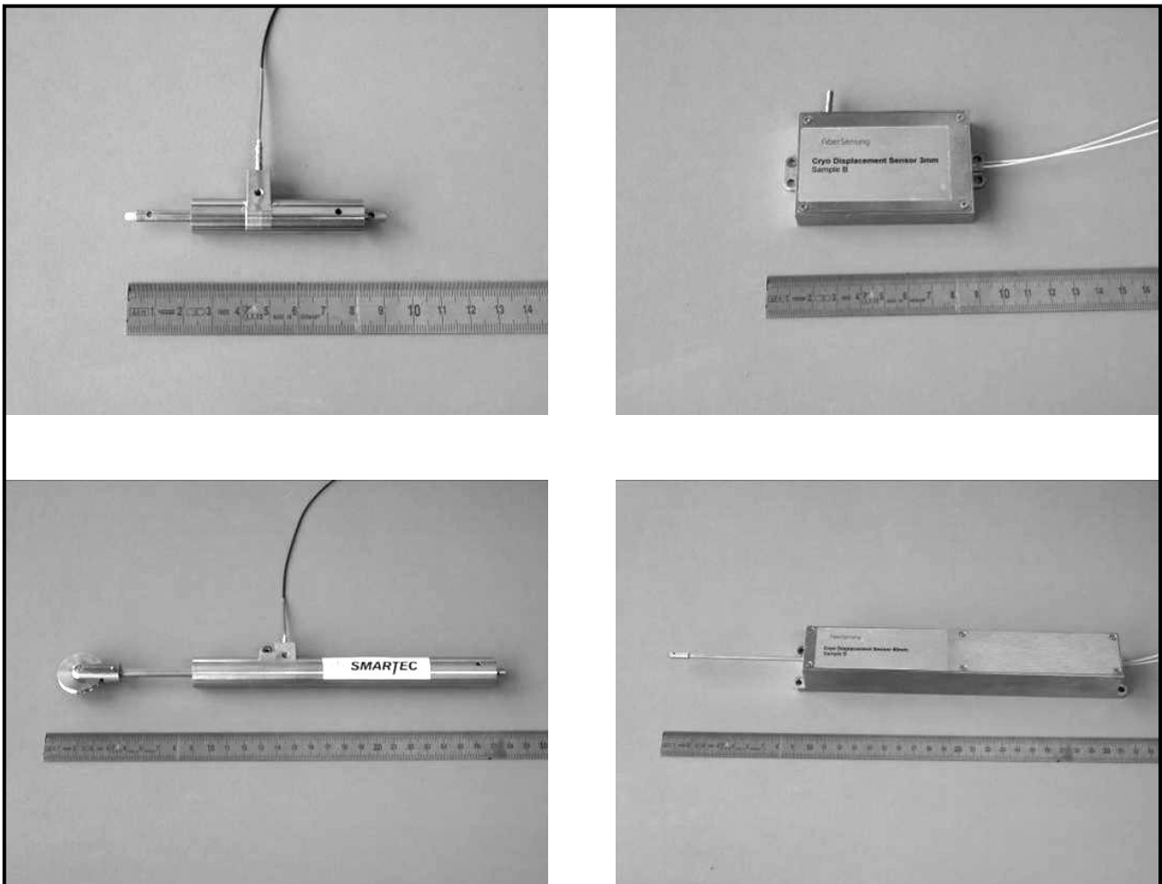
Figure 8. Fibre Optic displacement sensors, FP small displacement top left, FBG small displacement top right, FP large displacement bottom left, FBG large displacement bottom right
