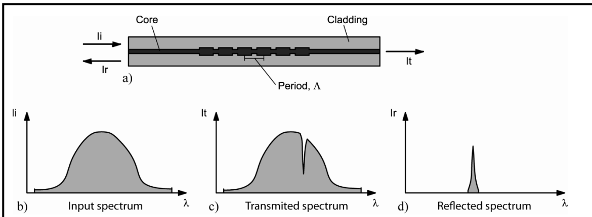
Figure 3. Functional principle of Fibre Bragg Grating sensors.
