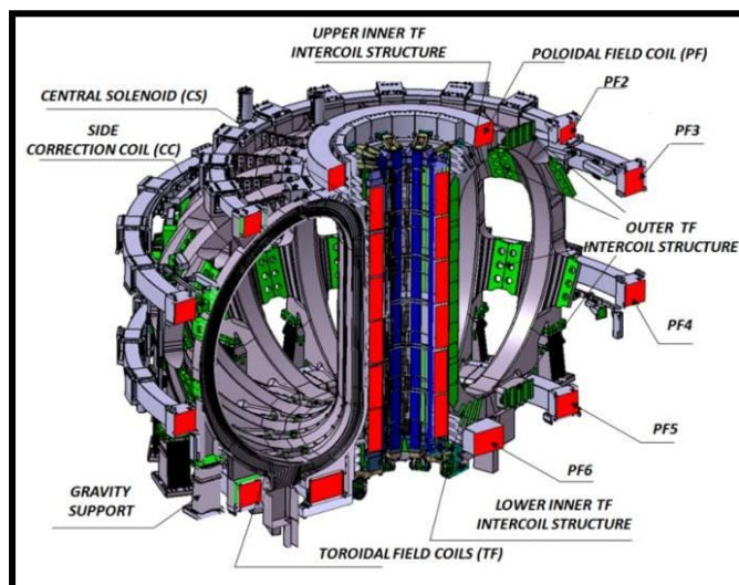
Figure 1. Overview of the ITER superconducting magnet system (feeder lines are not shown)
