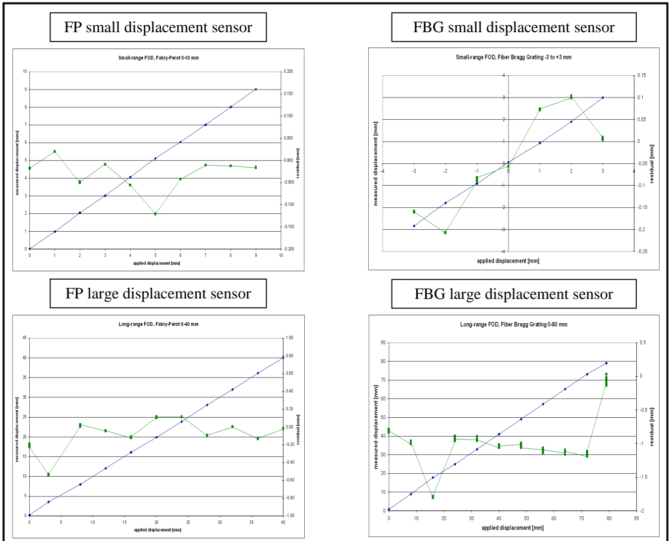
Figure 10. Displacement accuracy test results at nitrogen temperature. Sensor response and error compared to the true value are depicted for each type of sensor
