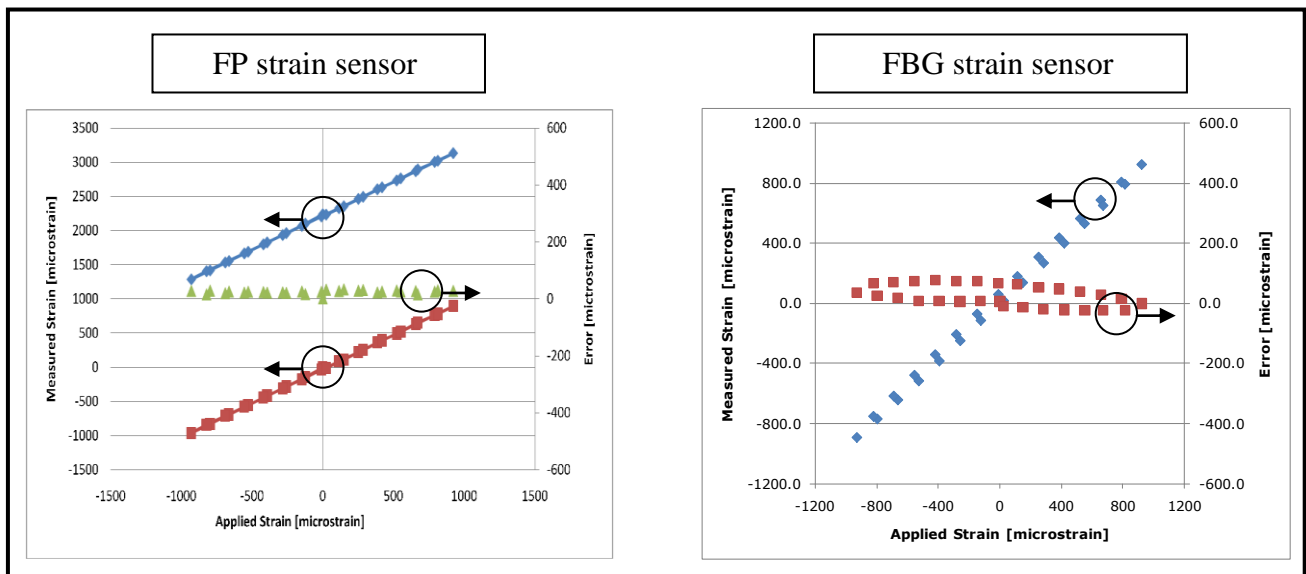
Figure 7. Strain accuracy test results at nitrogen temperature.
