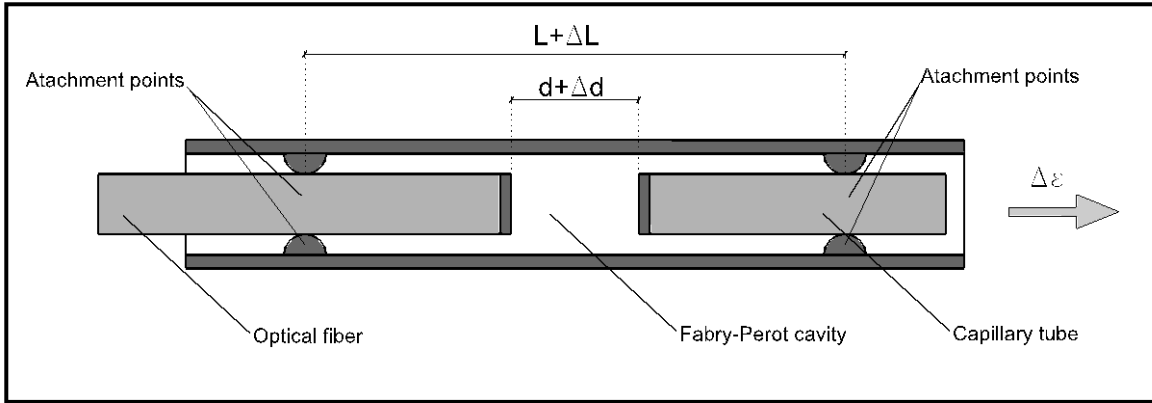
Figure 2: Functional principle of Fabry-Perot sensors.
