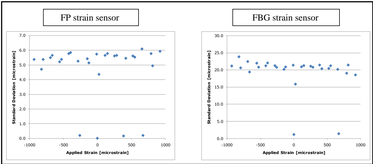
Figure 6. Strain resolution test results at nitrogen temperature.
