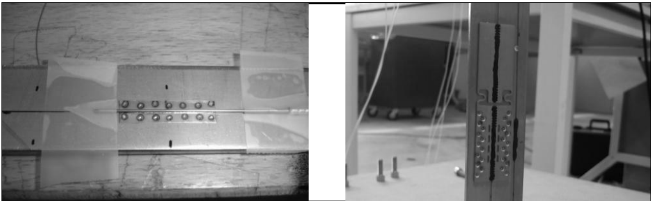
Figure 5. Fibre Optical strain sensors, FP left, FBG right, during testing.
