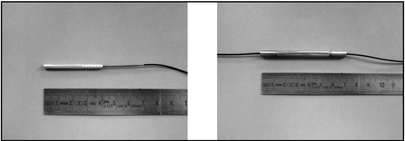
Figure 11. Fibre Optic temperature sensors, FP left, FBG right.
