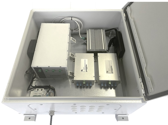
Outdoor enclosure including SOFO VII unit with two splitters and field PC.
