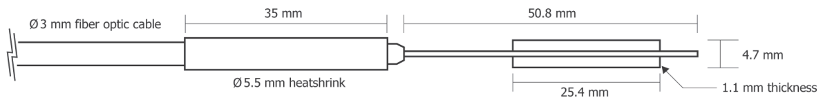
SFO-W Dimensions
